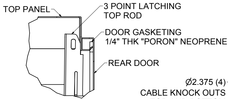
DETAIL D
