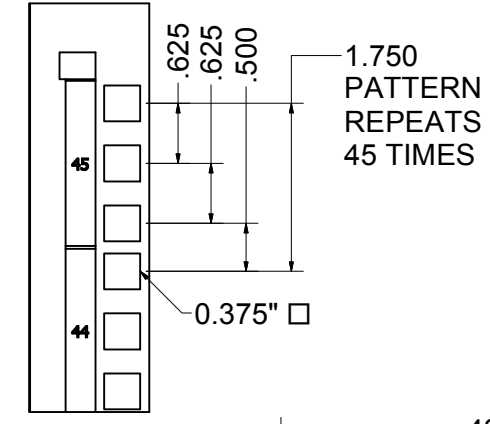
DETAIL C RAIL DETAIL
