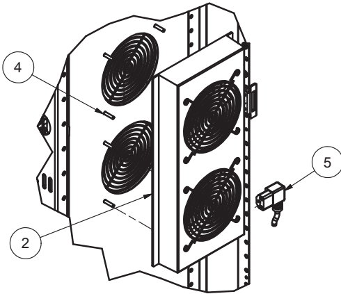
DETAIL B INSIDE OF DOOR
