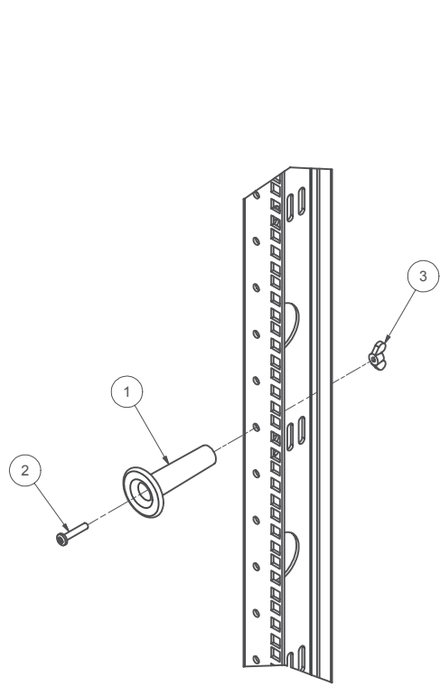
CMP INSTALLATION ON MOUNTING RAIL
