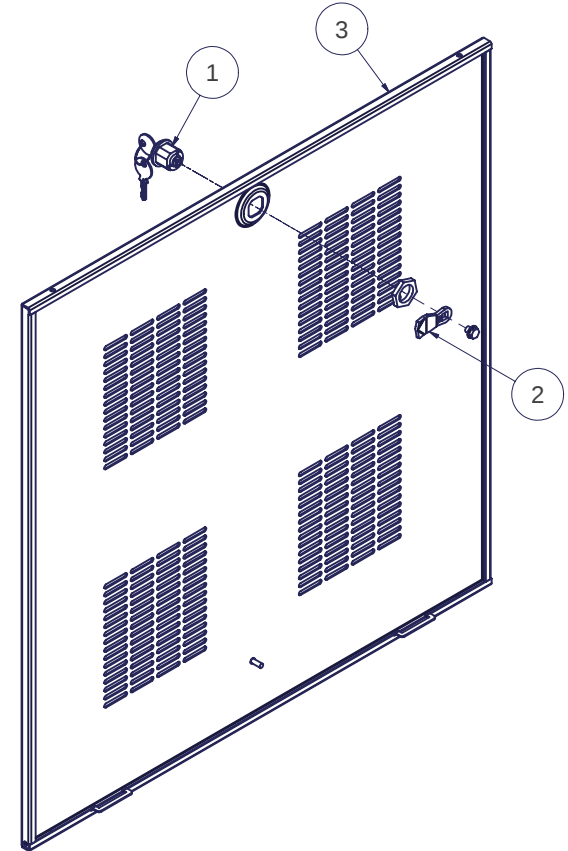
EXPLODED VIEW OF LOCK AND CAM (CAM SHOWN IN LOCKED POSITION)
