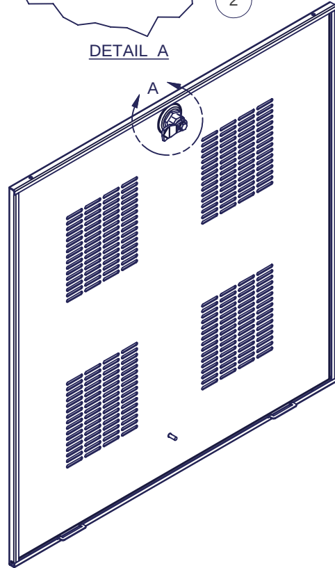
ASSEMBLED VIEW OF LOCK AND CAM (CAM SHOWN IN UNLOCKED POSITION)
