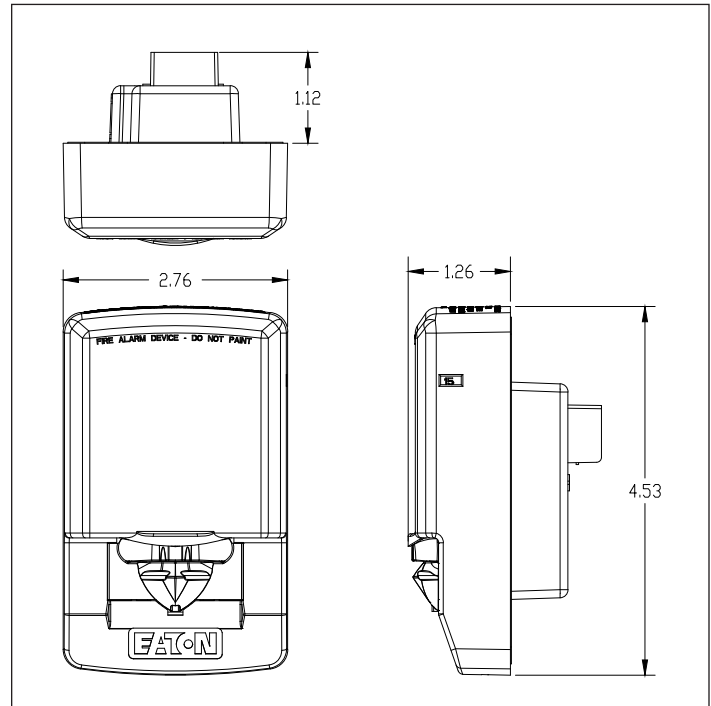
Figure 1. Wall Strobe
