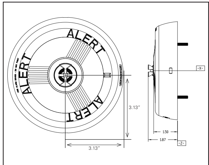
Figure 2. Ceiling Strobe
